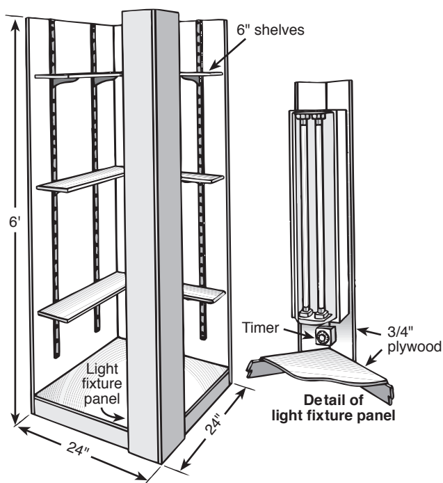
Figure 2. This homemade vertical lighting system with adjustable shelves can accommodate small or large plants.
